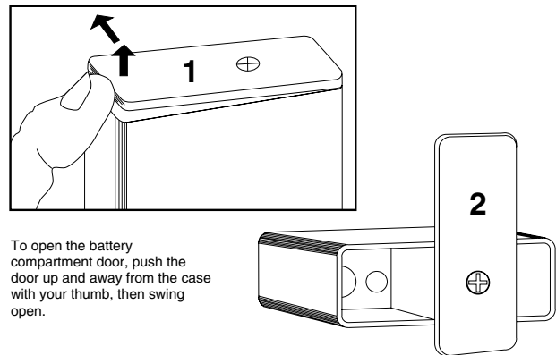
Figure 4 - Battery Replacement
