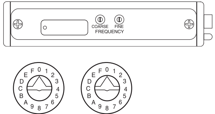
Figure 2 - Frequency Adjustment
