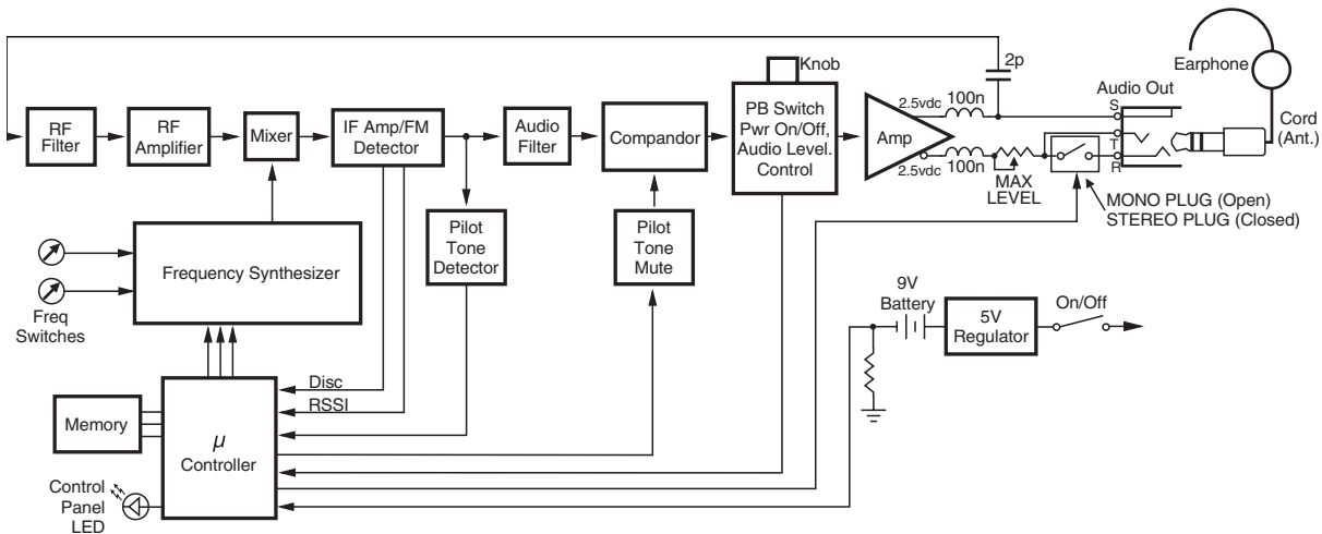
Figure 3 - R5a Block Diagram
